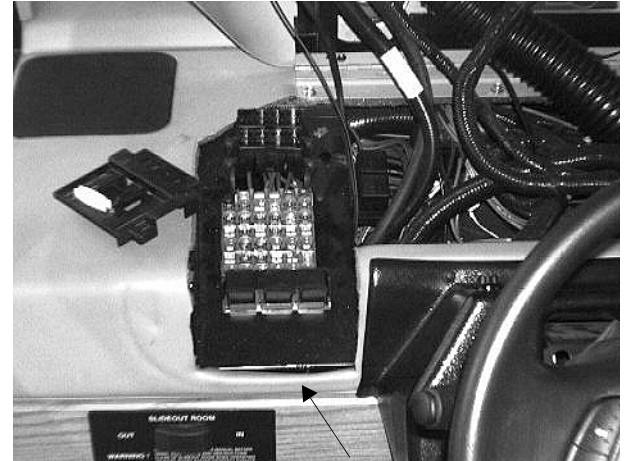
Automotive 12-Volt Fuse Block beneath lift-up dash pod
