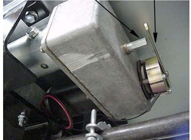
Slideout motor/gear assembly viewed from beneath coach
