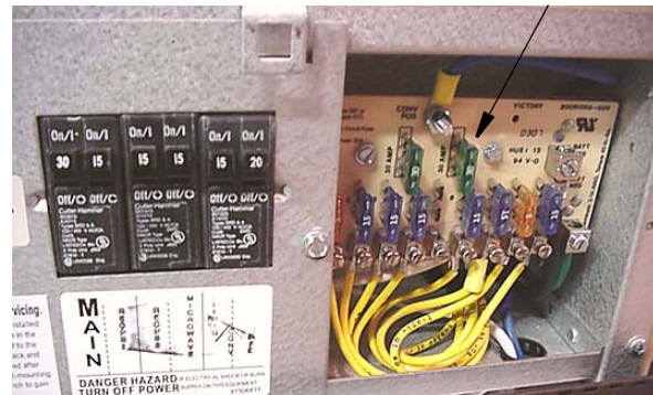
12-Volt House Fuses
