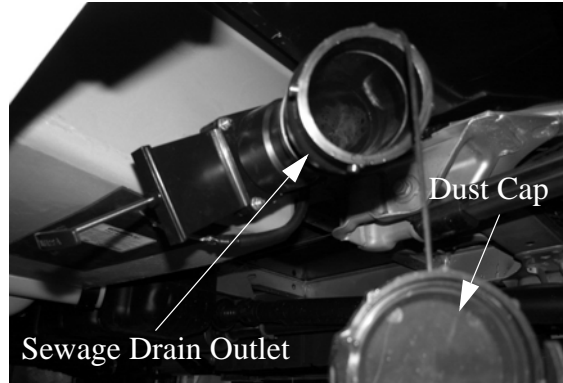
Sewage Drain Outlet (Located ahead of rear driver side wheel) -Typical View
