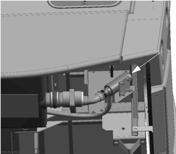
Waste Pump (Shown with panel removed) -Remove cap and manually turn waste pump shaft with a screwdriver
