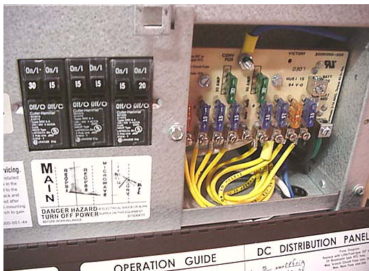
12V House Fuses -Typical View
