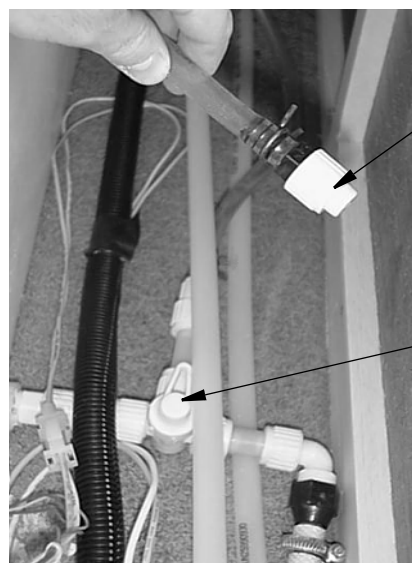
Antifreeze Siphon Tube and Winterization Valve -Typical View
