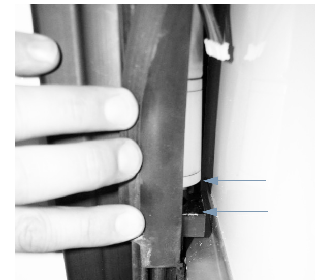
Slideout Motor (Located behind slideout wipe seal) • Use a screwdriver to push slideout motor UP (disengage).
