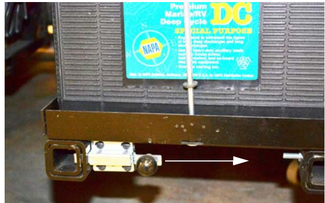
Pull locking device straight out (toward front end of coach) to release slide tray
