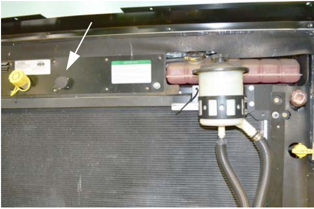
Diagnostic Plug (Located on rear engine compartment shroud) -Typical View
