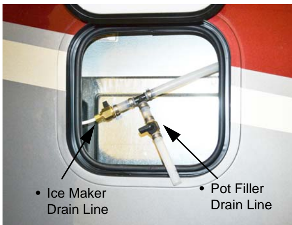
Pot Filler and Ice Maker Drain Line (Located in exterior Residential Refrigerator service compartment)
