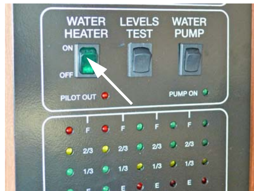
Gas Water Heater Switch (Located on Systems Monitor Panel)
