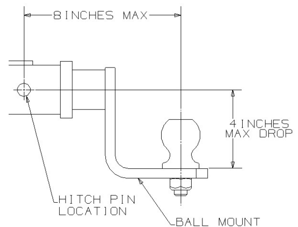
Hitch Assembly
