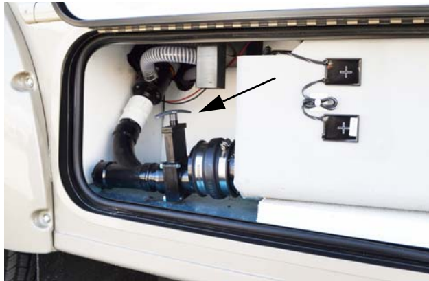
Gray Waste Tank Drain Valve (Located in driver side compartment behind rear wheel)
