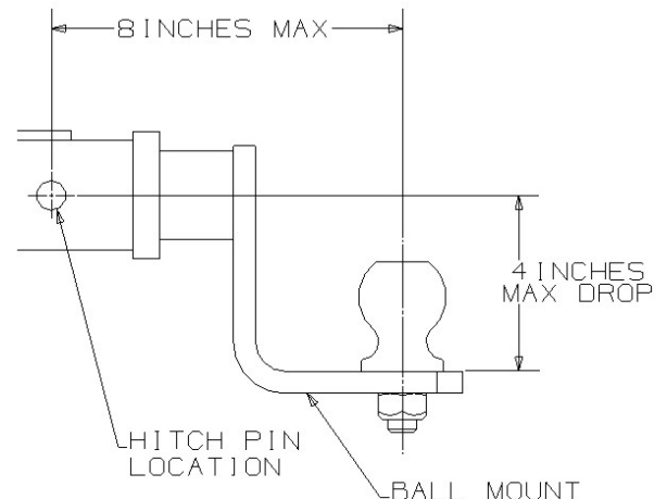
Hitch Assembly
