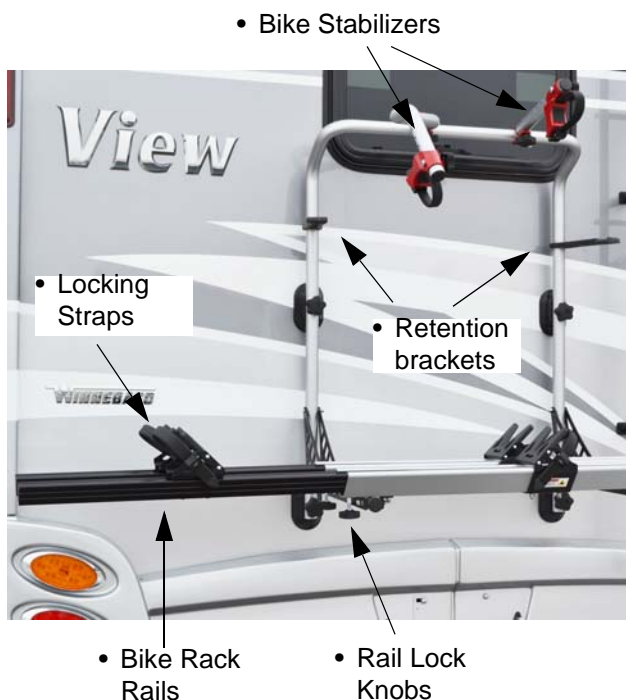
Bike Rack (shown in down position)
