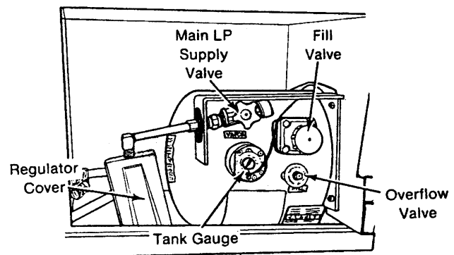
Typical LP Gas System Controls
