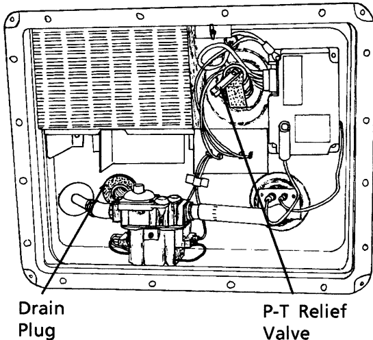
Water Heater Exterior Access
