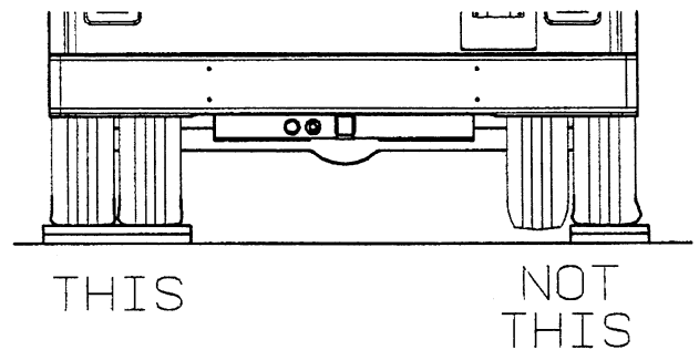
Blocking Rear Duals
