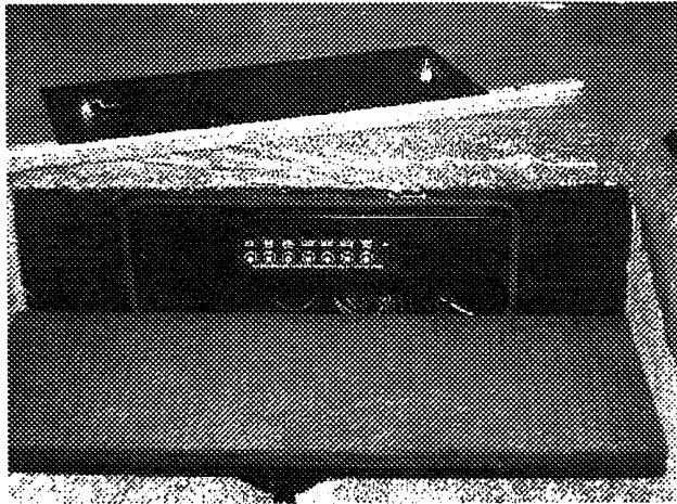
12-Volt Coach/Chassis System Breaker Panel behind carpeted panel of top step riser
