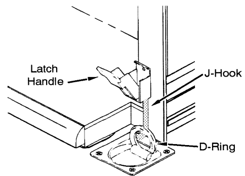
Travel Latches
