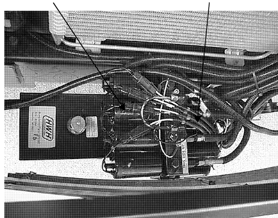
Leveling/Slideout System Hydraulic Pump (top view from hood opening)
