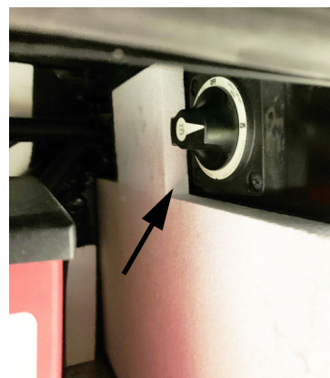
Inverter/charger disconnect switch. (Located inside the passengers compartment door near the Charger Unit) -Typical View
